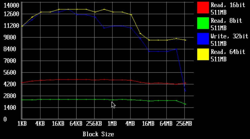
Memory speed (MB/Sec. per Block Size)
